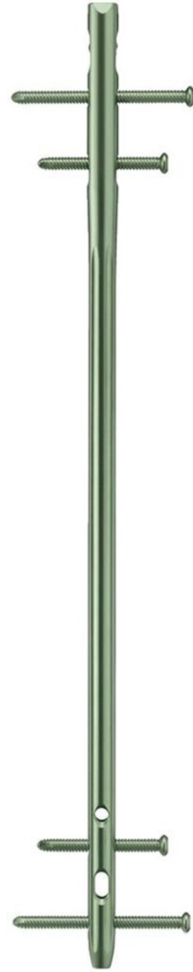
antegrade R/AFN, 300–480 mm antecurvature 1500 mm
